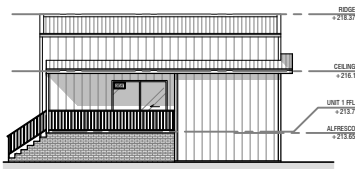
NORTHERN ELEVATION NTS
