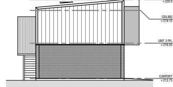
WESTERN ELEVATION NTS
